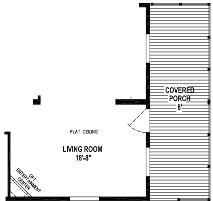
OPTION PORCH/ALTERNATE ENTRY
